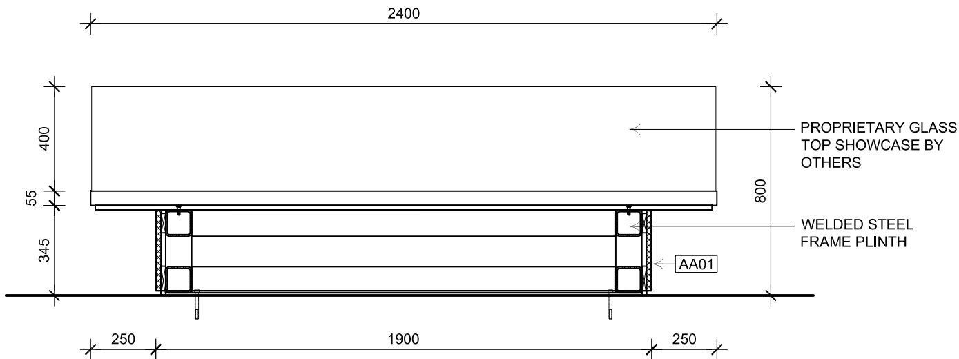
AA SECTION 1:20
