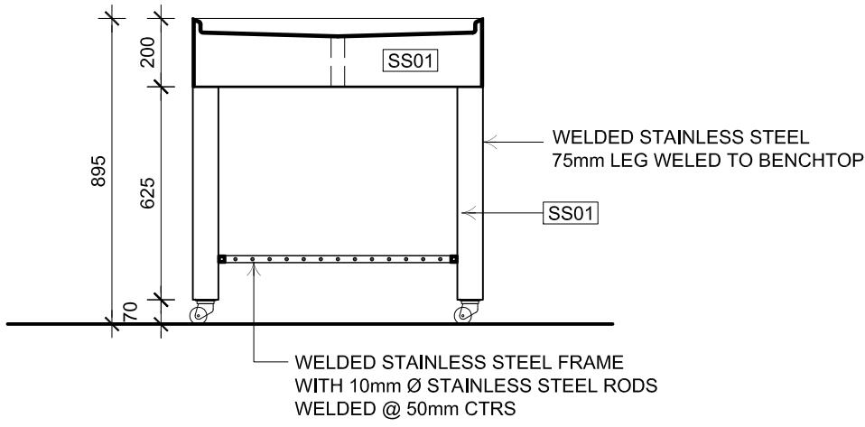
AA SECTION 1:20
