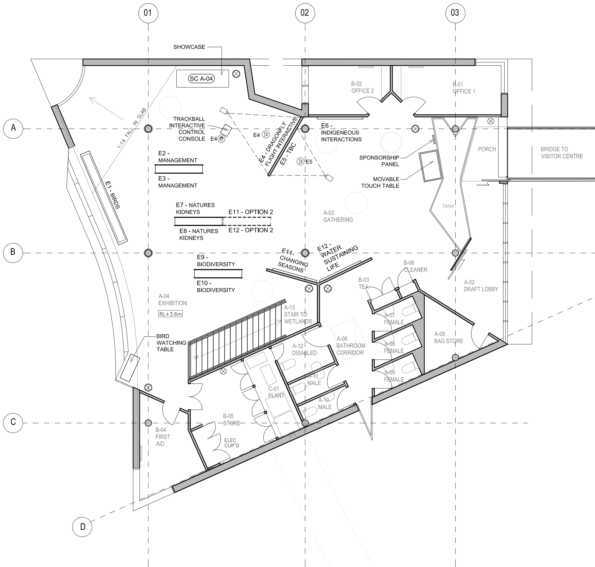
01 FLOOR PLAN 1:100
