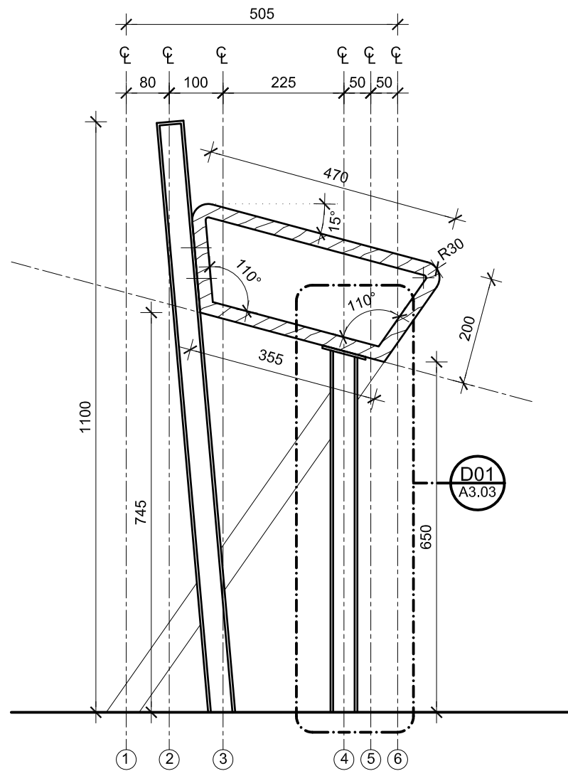
EE SECTION - 1:10
