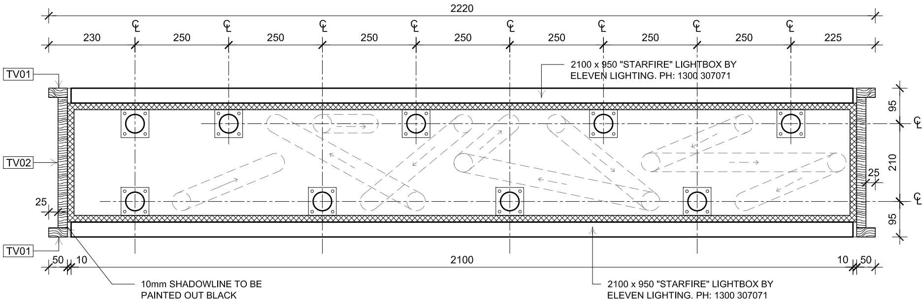
CC SECTION A3.02 1:10
