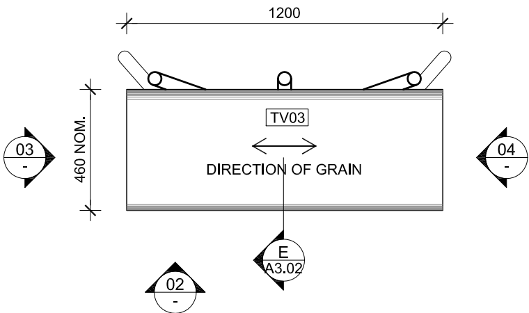
01 PLAN (BIRD WATCHING TABLE) - 1:20
