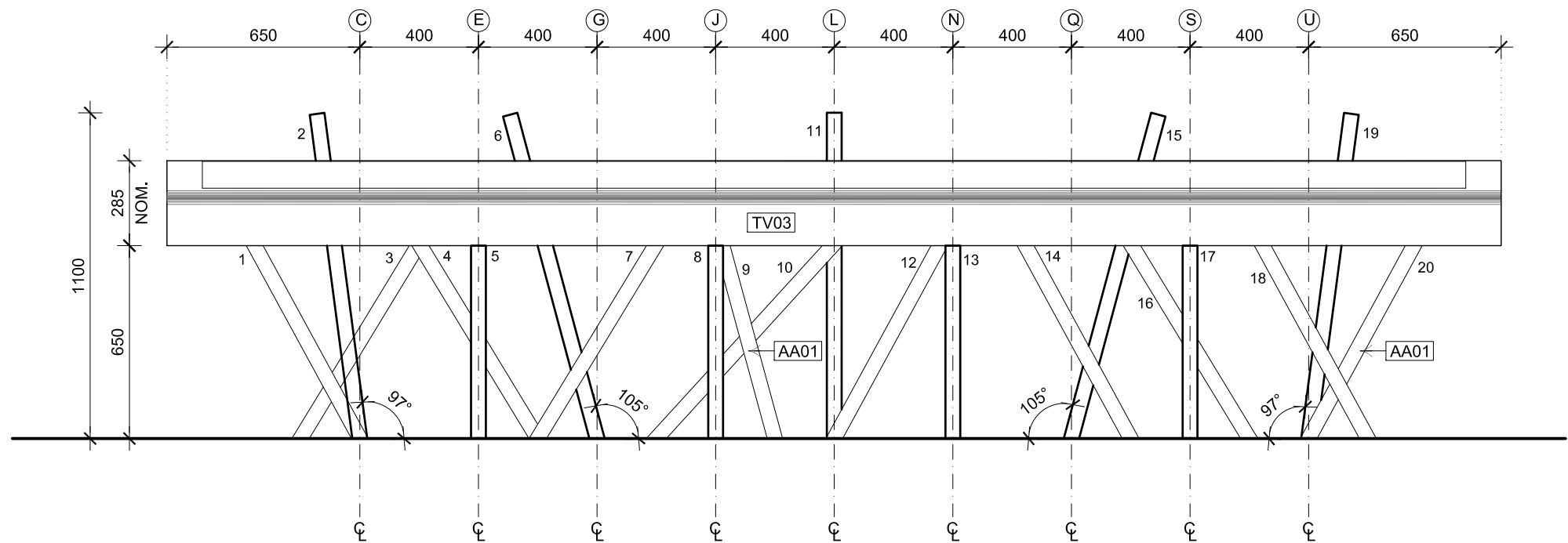
02 FRONT ELEVATION 1:20
