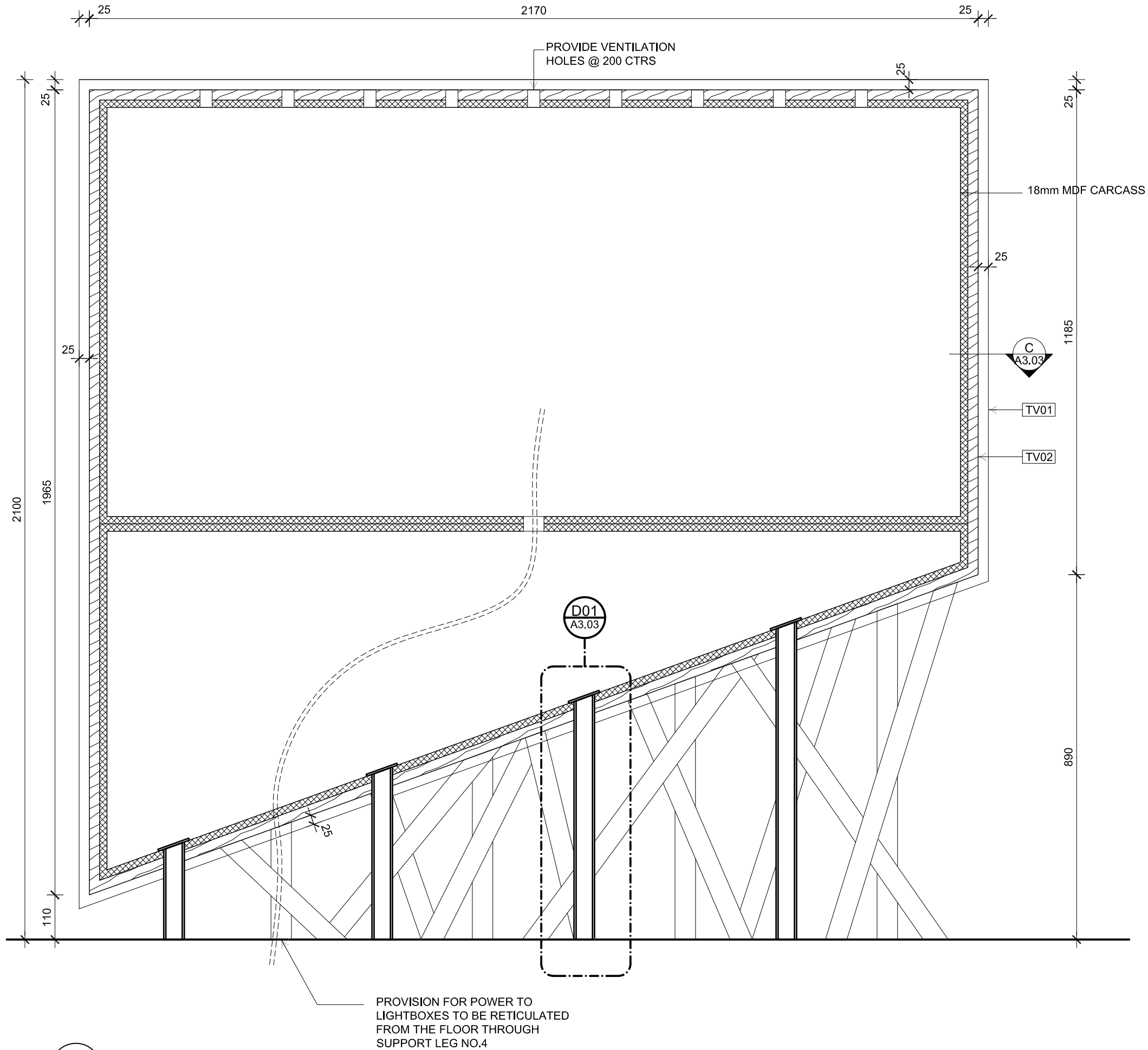
AA SECTION A3.01 1:10
