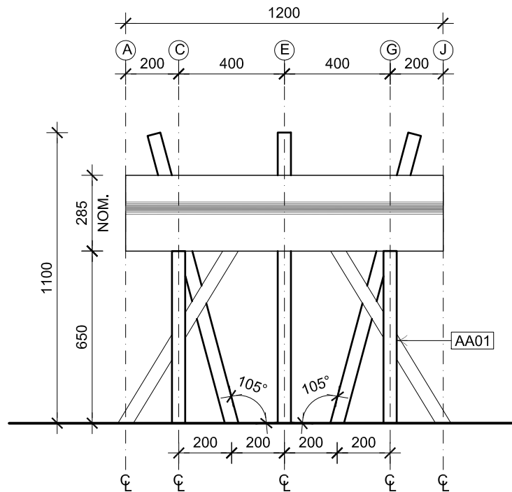
02 FRONT ELEVATION - 1:20
