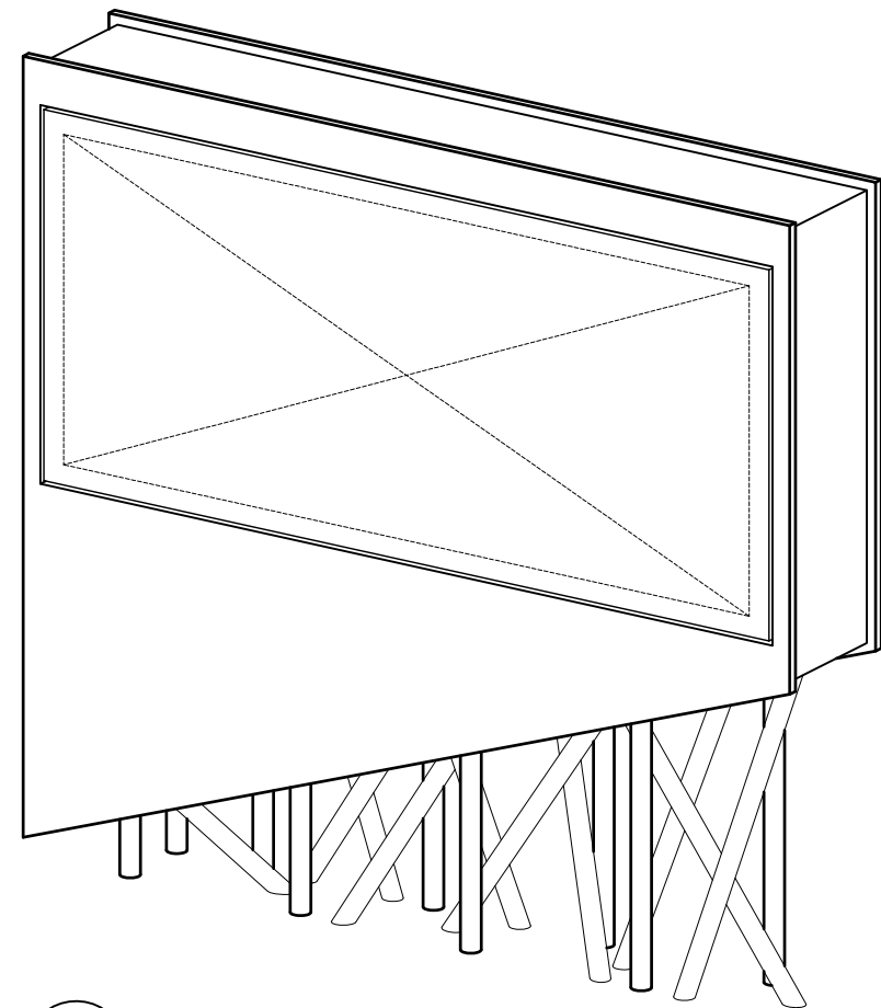
02 ISOMETRIC VIEW - 1:10
